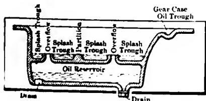
Fig. 6—The oil reservoir of the Moon car is formed by the base-chamber of the motor
